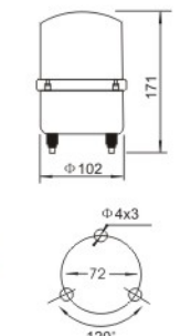
LTE-1103 Straight Type
