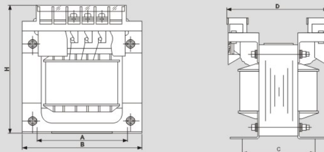
Outline of control transformer of BK2-25~200
