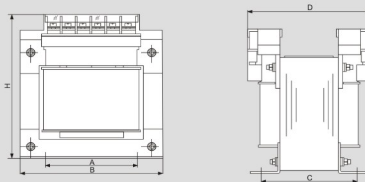
Outline of control transformer of BK2-250~1000
